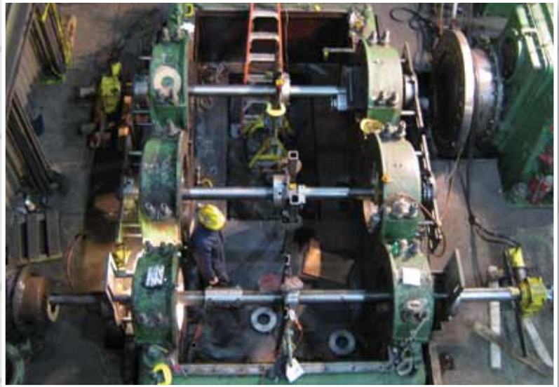
Line Boring
