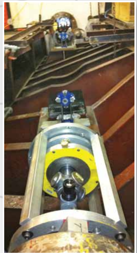
In-Shop Testing of Laser Tracker
