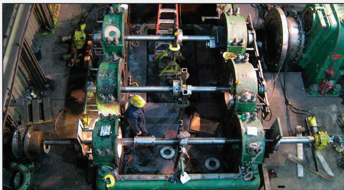
On-Site Line Boring Field Machining
