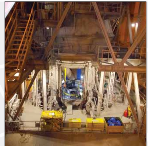
Cement Mill Grinding Table Field Machining
